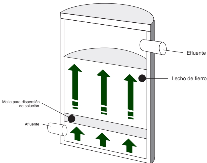
Figura 5.2: Esquema de cartucho de recuperación (The Silver Council, 1997a; 1997b; 1997c)
